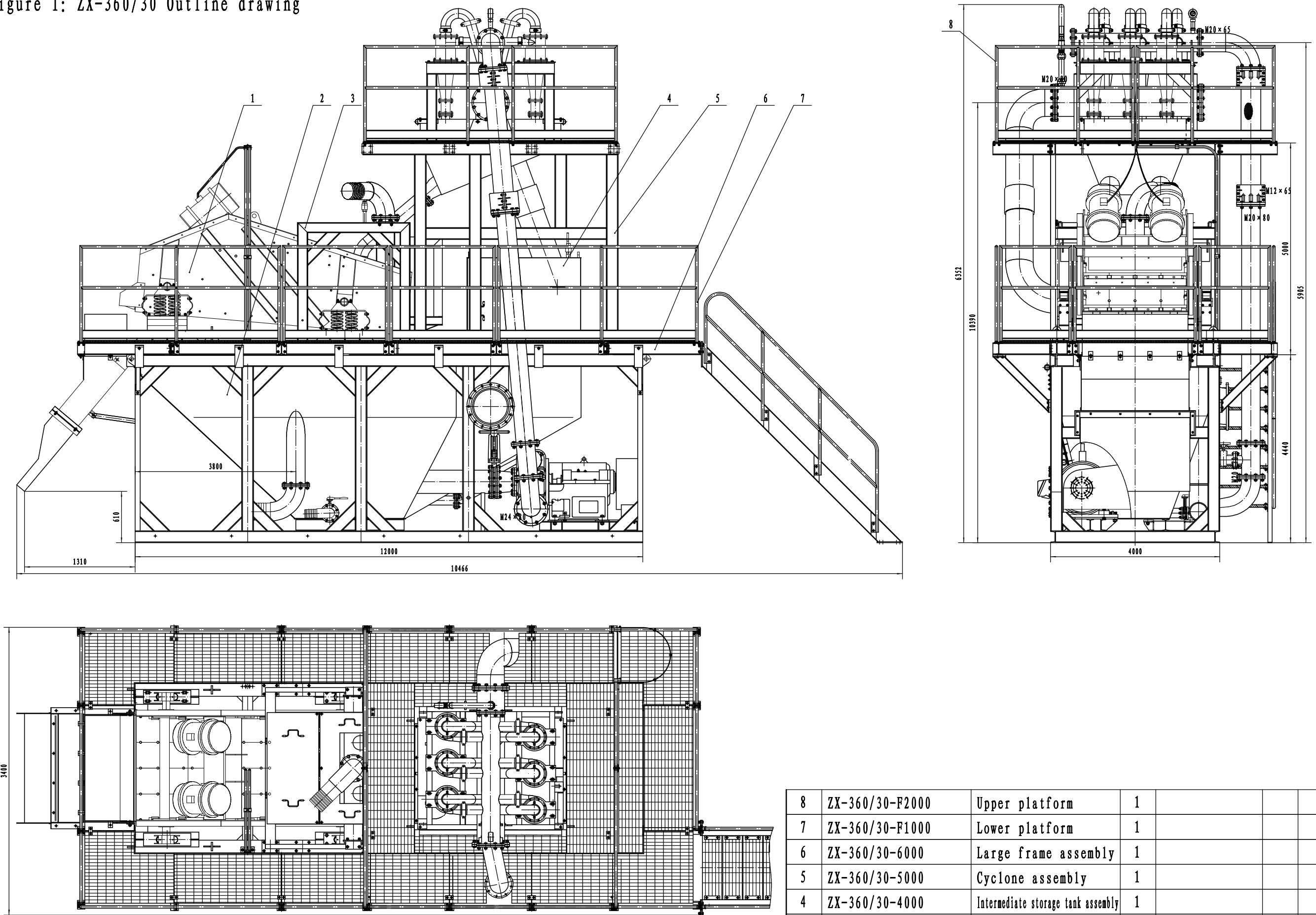
Figure 1: ZX-360/30 Outline drawing
